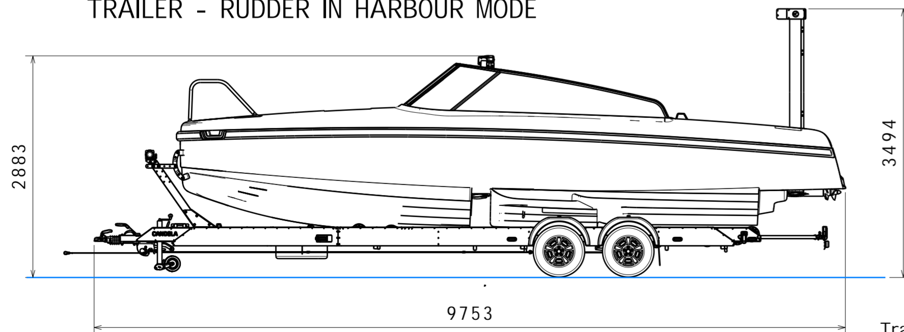
TRAILER - RUDDER IN HARBOUR MODE
